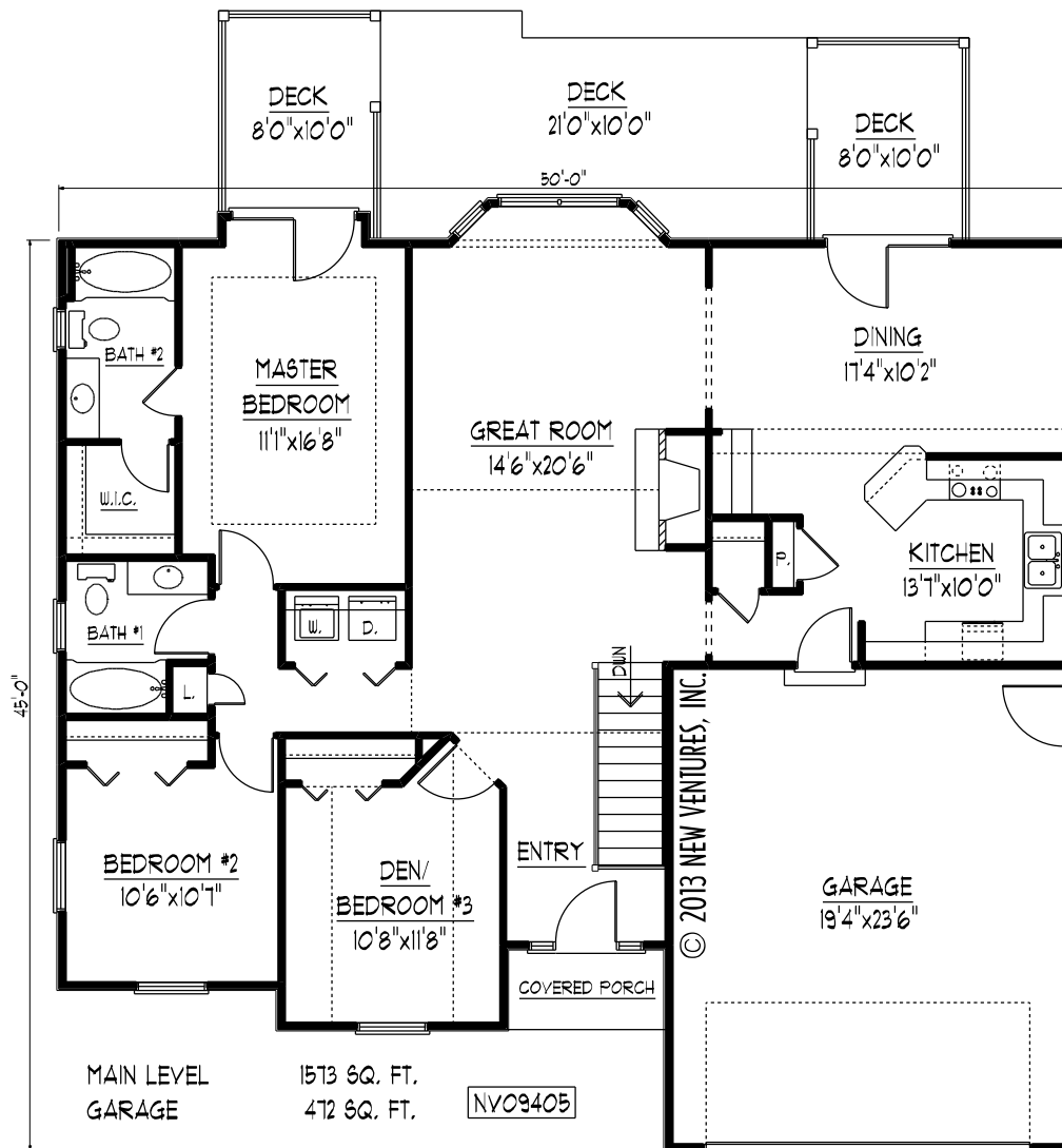
MAIN LEVEL FLOOR PLAN
