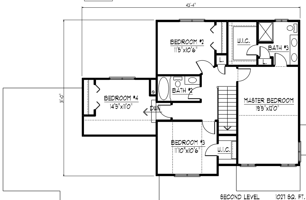
NV09103 SECOND LEVEL FLOOR PLAN
