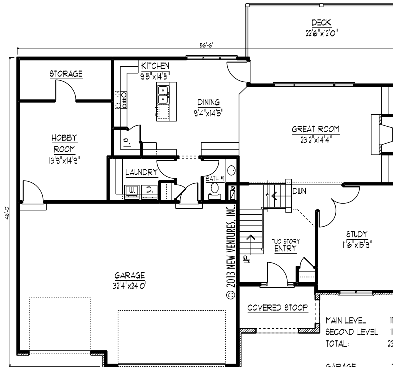
MAIN LEVEL FLOOR PLAN
