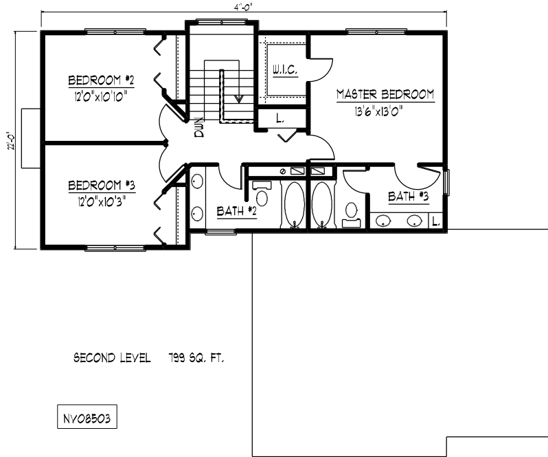
SECOND LEVEL FLOOR PLAN
