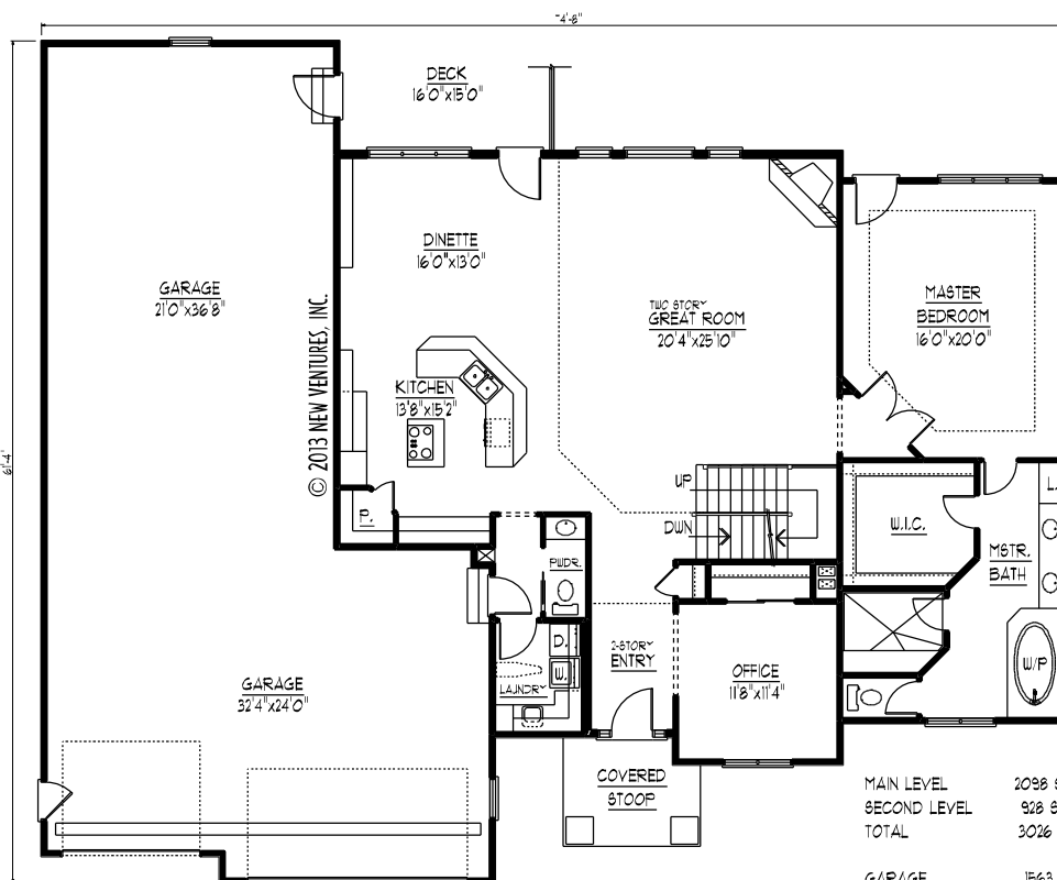
MAIN LEVEL FLOOR PLAN
