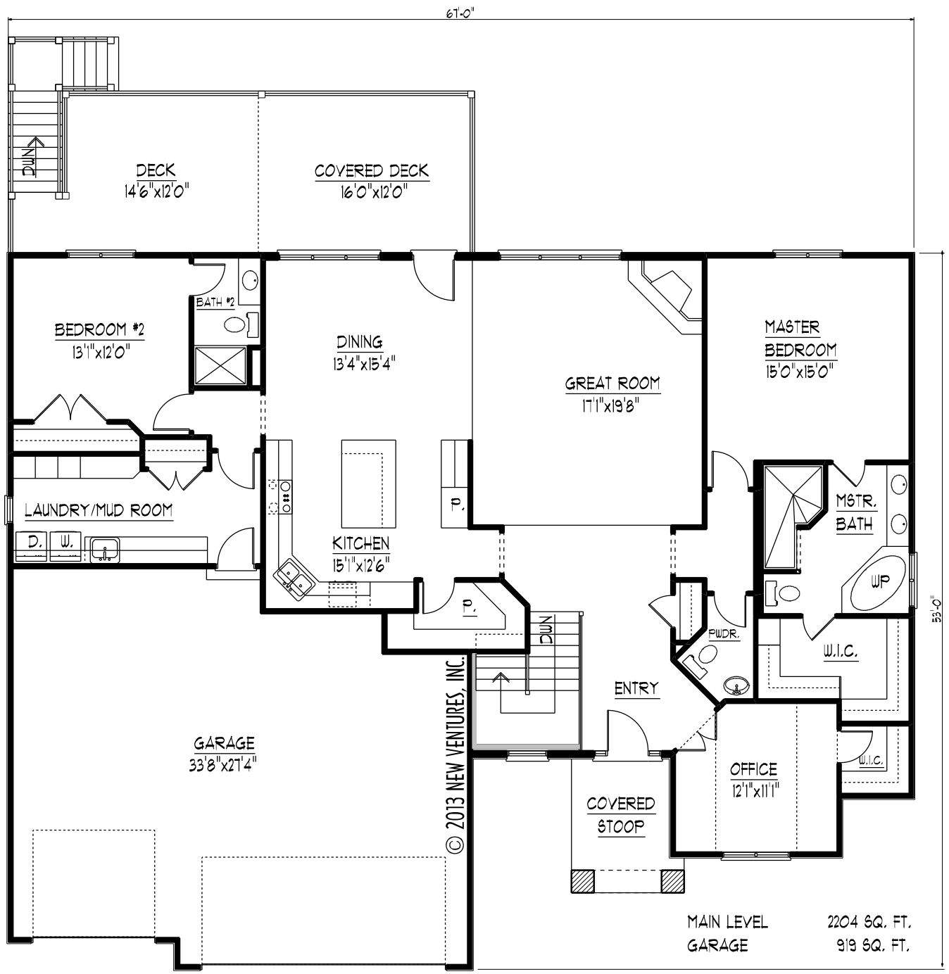
MAIN LEVEL FLOOR PLAN NV08011
