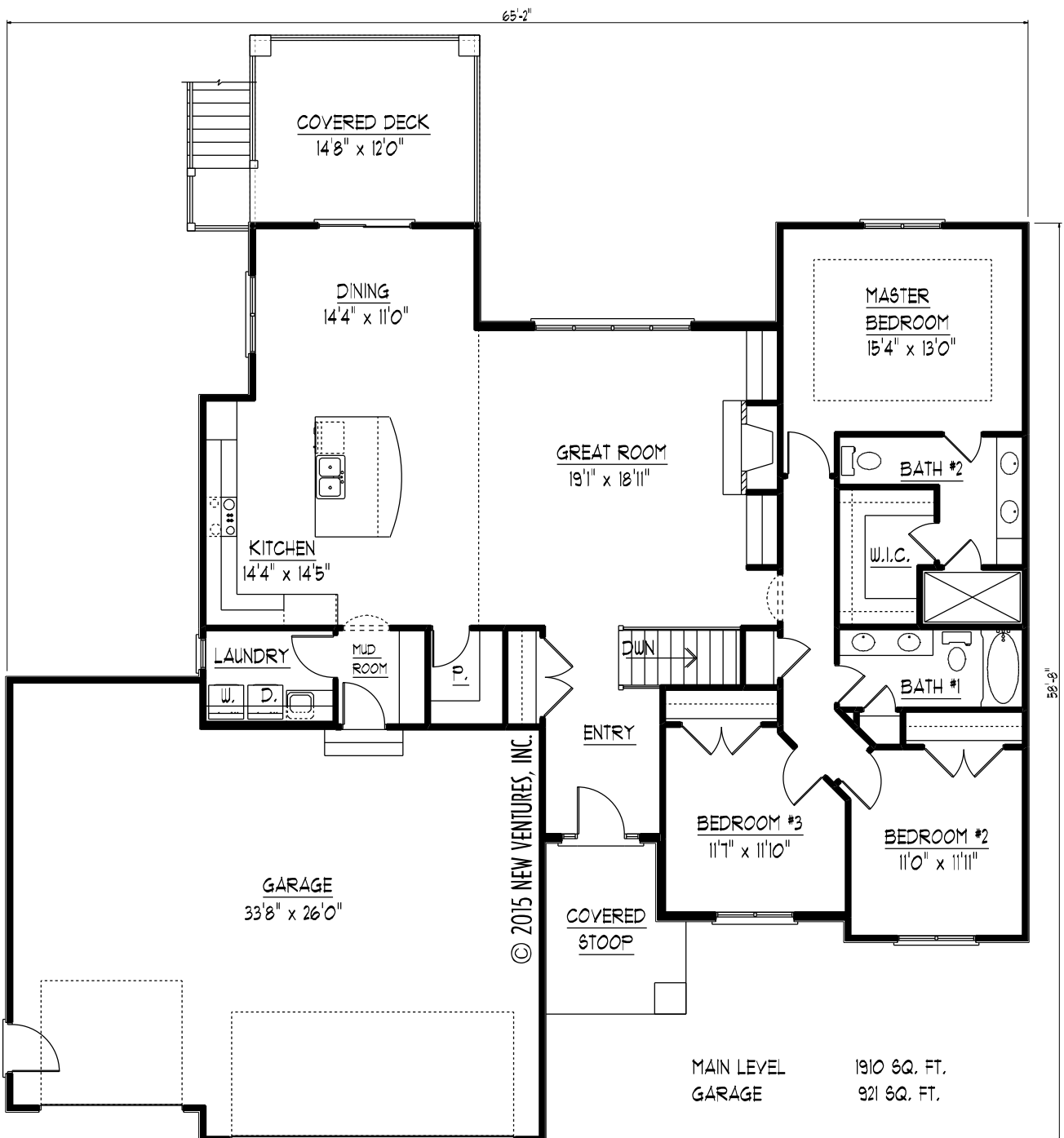
MAIN LEVEL FLOOR PLAN NV06812
