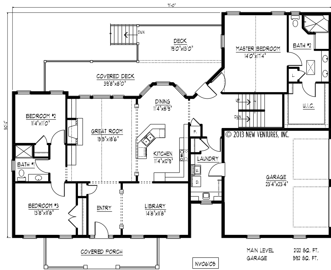
MAIN LEVEL FLOOR PLAN
