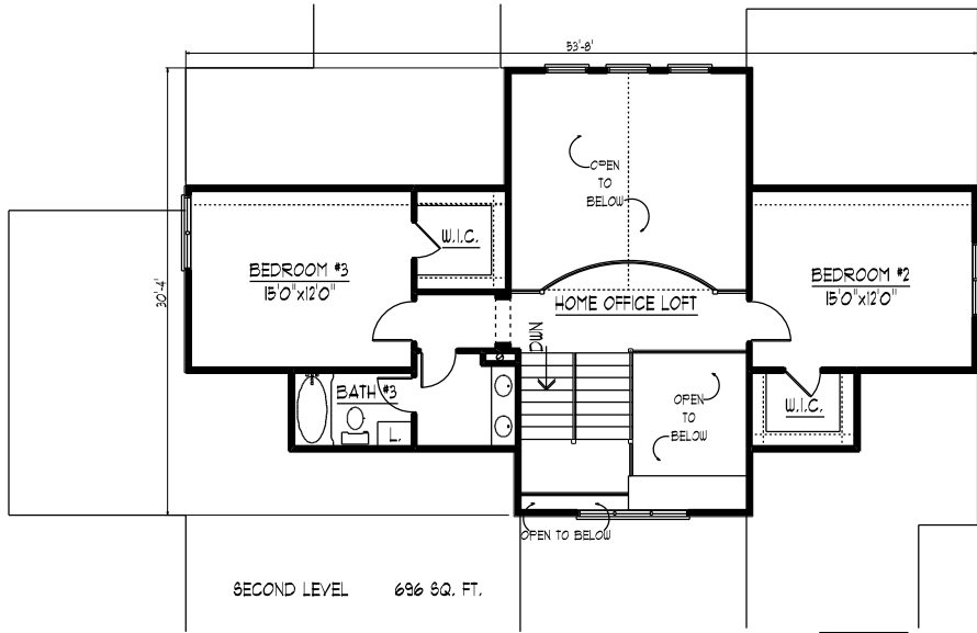
SECOND LEVEL FLOOR PLAN
