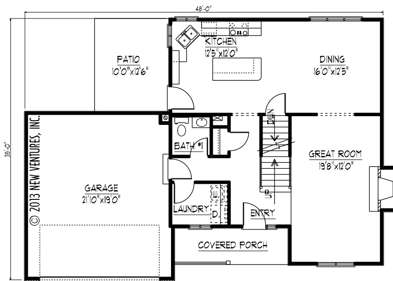
MAIN LEVEL FLOOR PLAN
