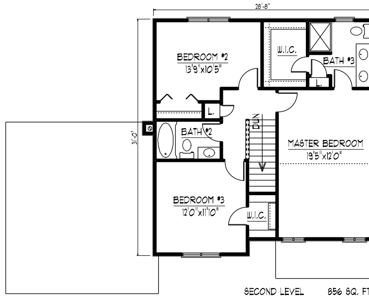
SECOND LEVEL FLOOR PLAN
