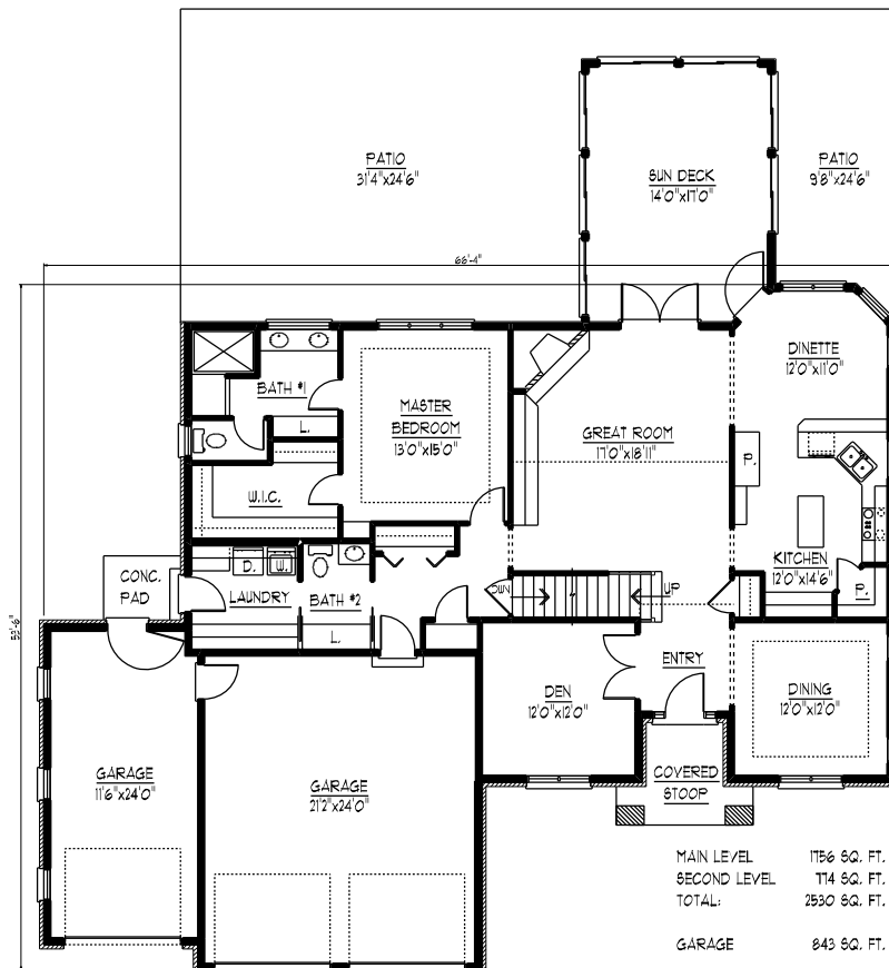
MAIN LEVEL FLOOR PLAN NV03806
