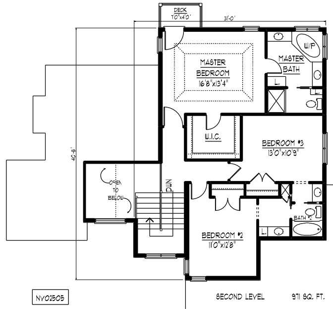
SECOND LEVEL FLOOR PLAN
