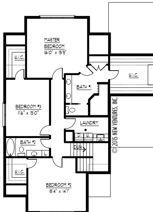
SECOND LEVEL FLOOR PLAN NVO2012
