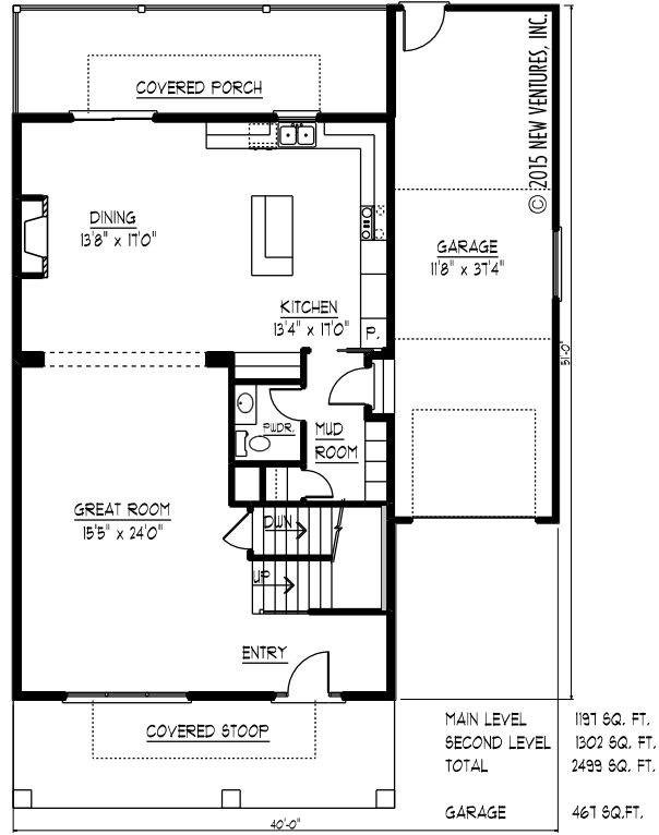
MAIN LEVEL FLOOR PLAN NVO2012
