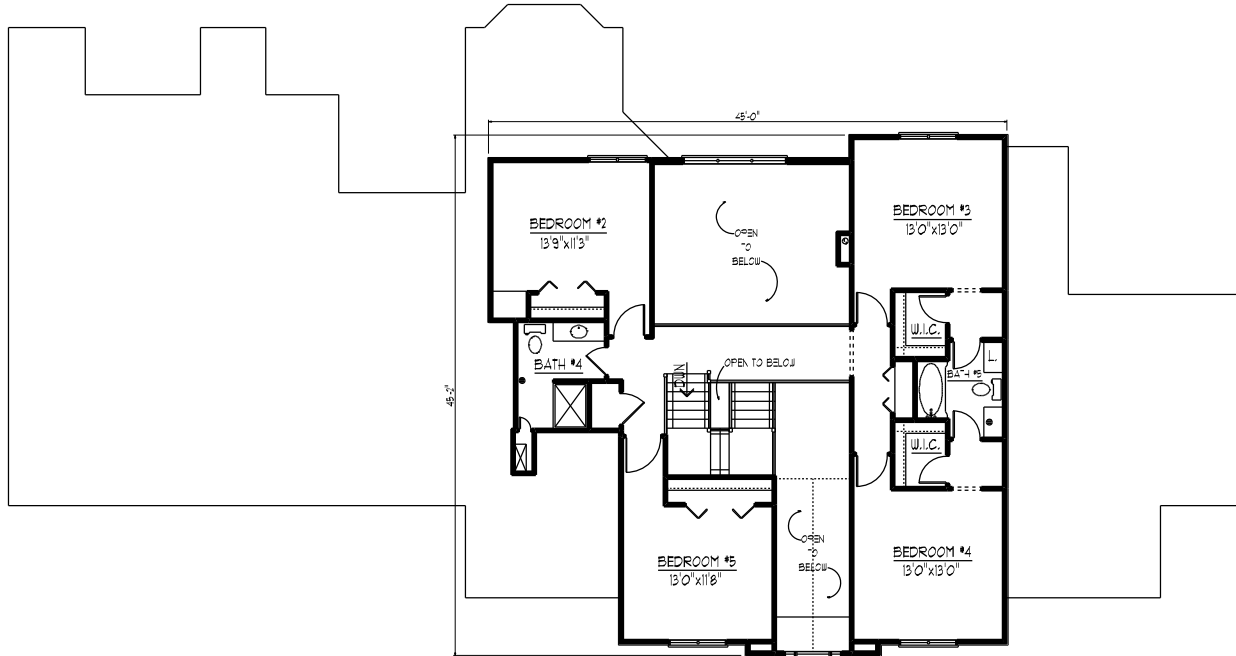
SECOND LEVEL FLOOR PLAN
