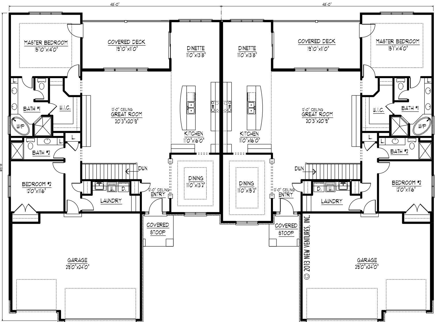
MAIN LEVEL FLOOR PLAN
